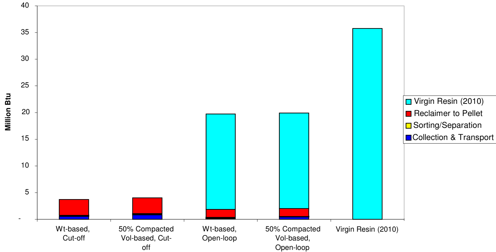
Figure 3-2a. Energy Results by Life Cycle Stage for Production of Recycled HDPE Resin Pellet (million Btu per 1,000 pounds of resin)
